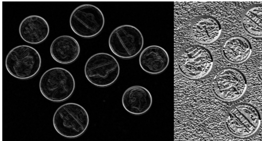
Gradient Magnitude, G_{mag} (left), and Gradient Direction, G_{dir} (right), us
